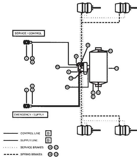
TA-8000 Series Tandem Axle
